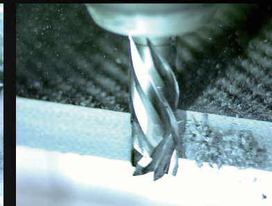
Side cutting
