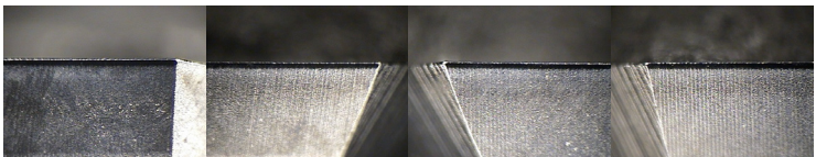
1. Tooling pictures after Trimming cutting testing
