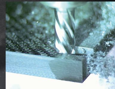
Slotting
