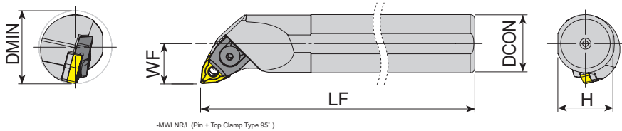
..MWLNR/L (Pin + Top Clamp Type 95°)
